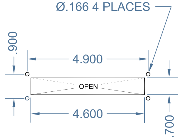
PANEL CUTOUT
